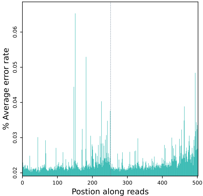
Error rate distribution along reads (R10215)
